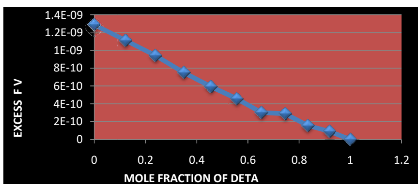
Fig 10 Graph between variation of excess free volume and mole fraction of DETA in 1-Chloronaphthalene at constant temperature and fixed ultrasonic frequency
