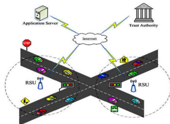
Figure 1: Architecture of VANET
