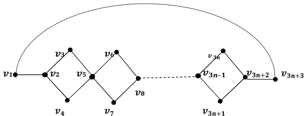
Figure 5: Vertex odd mean labeling of nC_4+P_4
