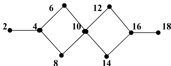
Figure 10: Vertex even mean labeling of 2C_4 + 2P_2
