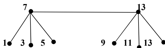
Figure 2: Vertex odd mean labeling of P_2 + 2S_3
