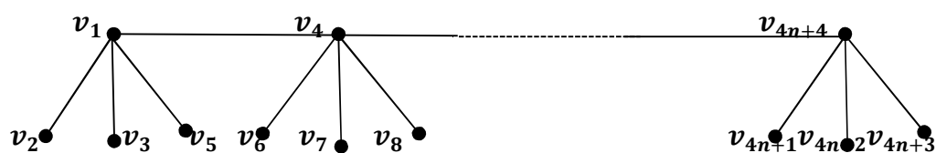
Figure 1: Vertex odd mean labeling of P_n + nS_3
