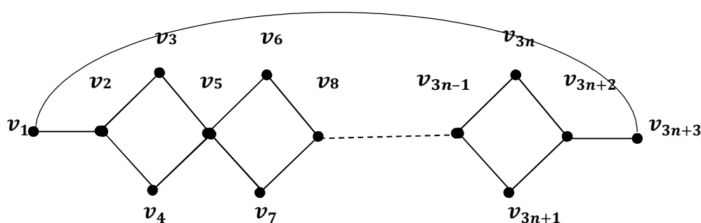
Figure 11: Vertex even mean labeling of nC_4 + P_4
